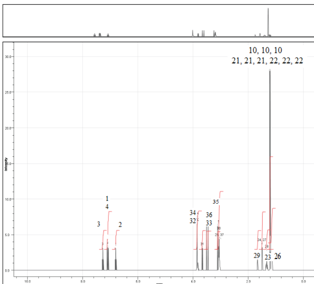
Figure 38: Better resolution of ^1\text{H} -NMR spectrum of (AZ-2) by Marvin Sketch.
